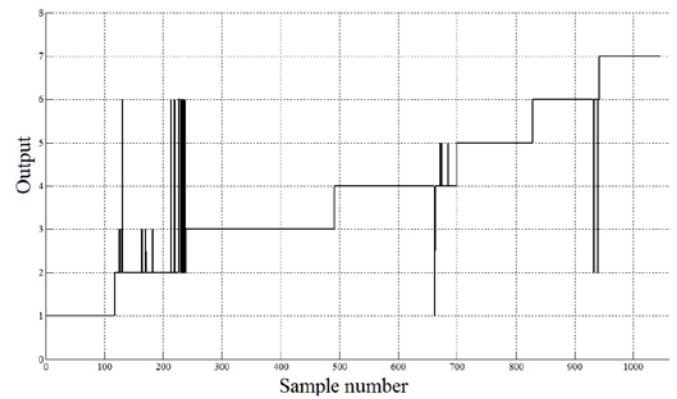
Fig. 2. Response of the artificial neural network with sigmoid activation function and 7 neurons in the hidden layer- Classification method
